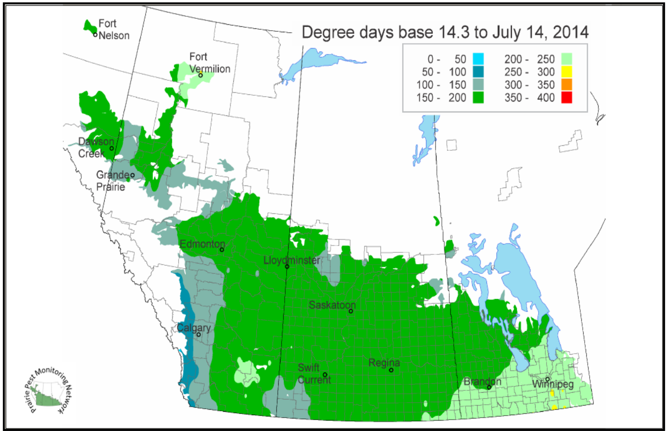
Figure 3 - Degree day accumulations, as of Week 28, across the Prairie Provinces.
