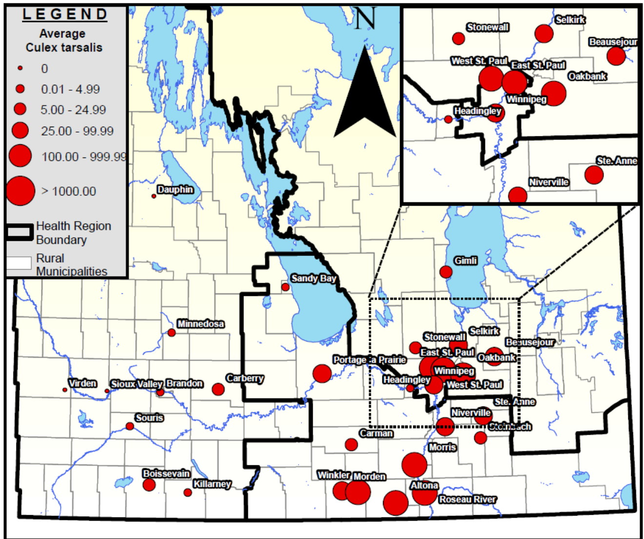
Figure 2 – Average number of Culex tarsalis mosquitoes collected across southern Manitoba during Week 28.
