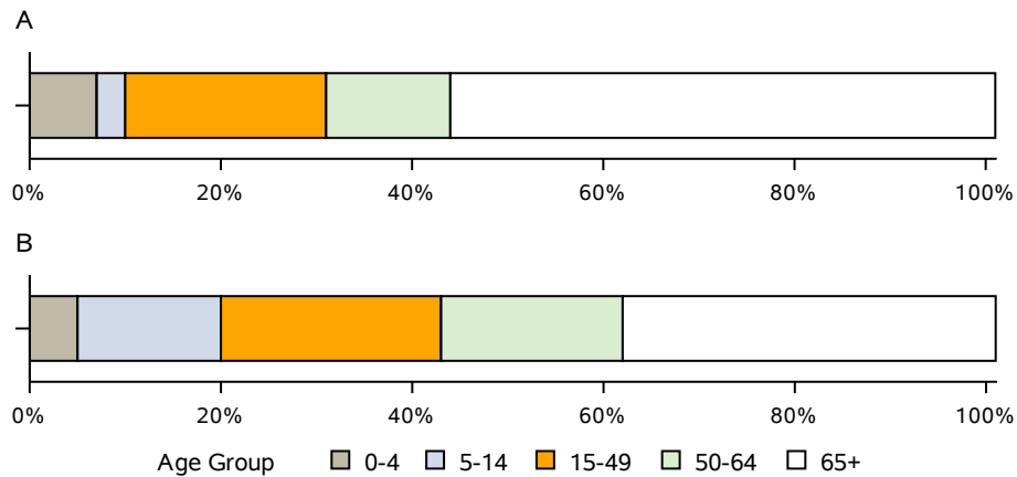
Figure 2. Distribution of Influenza Cases since September 1, 2017 by Age Group, Manitoba, 2017–2018
